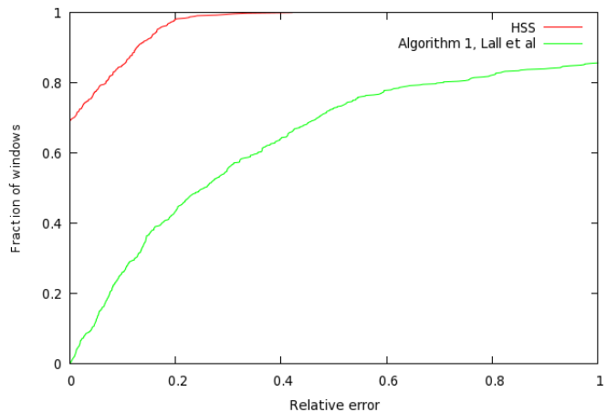
(b) H(Y|X) , 40,000 counters
