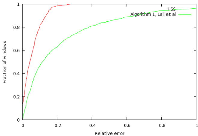
(a) H(X|Y) , 40,000 counters
