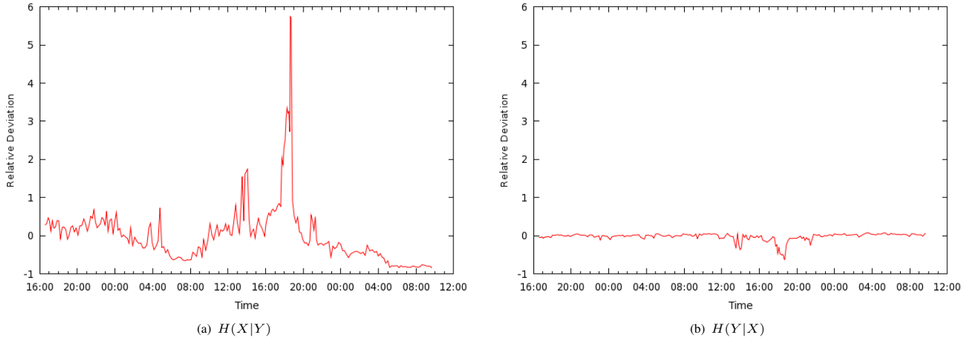
Fig. 7: Relative deviation of conditional entropy estimates from median, X \equiv Frame length, Y \equiv Src MAC
