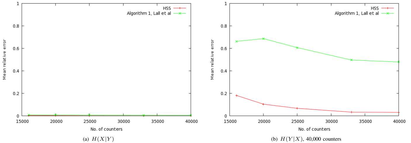
Fig. 6: Mean relative error with varying numbers of counters, X \equiv Frame length, Y \equiv Duration/ID
