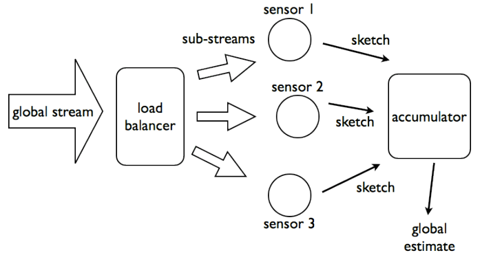
Fig. 2: Distributed monitoring of (conditional) entropy using sketching.
