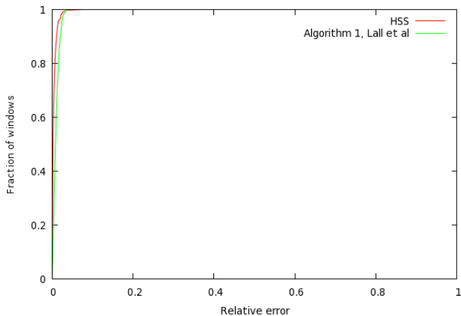
(a) H(X|Y) , 16,000 counters
