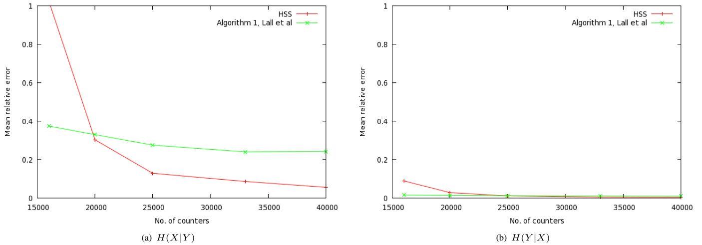
Fig. 5: Mean relative error with varying numbers of counters, X \equiv Frame length, Y \equiv Src MAC
