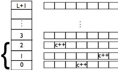
Fig. 1: The HSS sketch. The levels a certain item is propagated to are marked by the brace. The corresponding counters incremented are marked “c++”.
