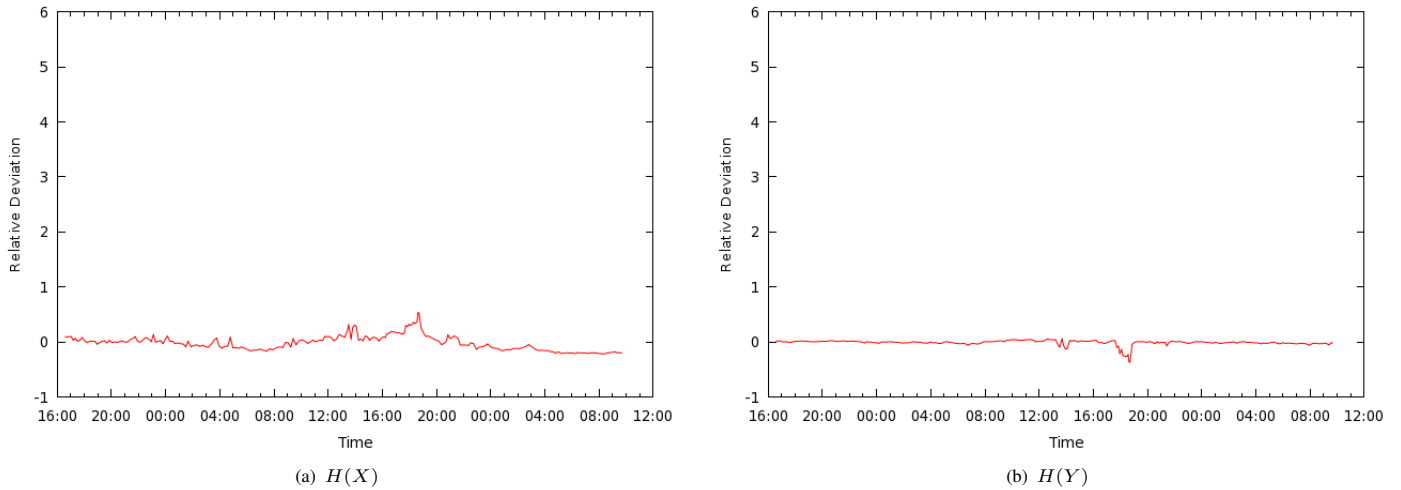
Fig. 8: Relative deviation of entropy estimates from median, X \equiv Frame length, Y \equiv Src MAC
