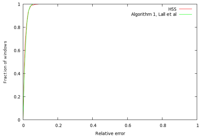
(b) H(Y|X) , 25,000 counters
